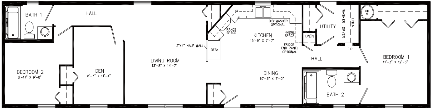
16 X 72 - 3252 (NOT AVAILABLE IN 14' WIDE) | 1152 SQ. FT.
