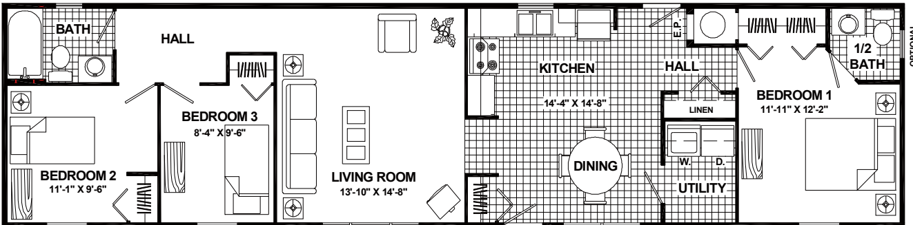
16 X 67 - 3248 (AVAILABLE IN 14' WIDE) 1072 SQ. FT.
