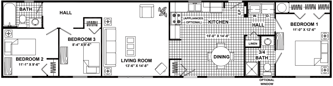
16 X 67 - 3247 (AVAILABLE IN 14' WIDE) 1072 SQ. FT.
