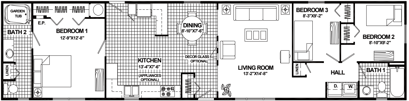
16 X 72 - 3293 (NOT AVAILABLE IN 14' WIDE) | 1152 SQ. FT.
