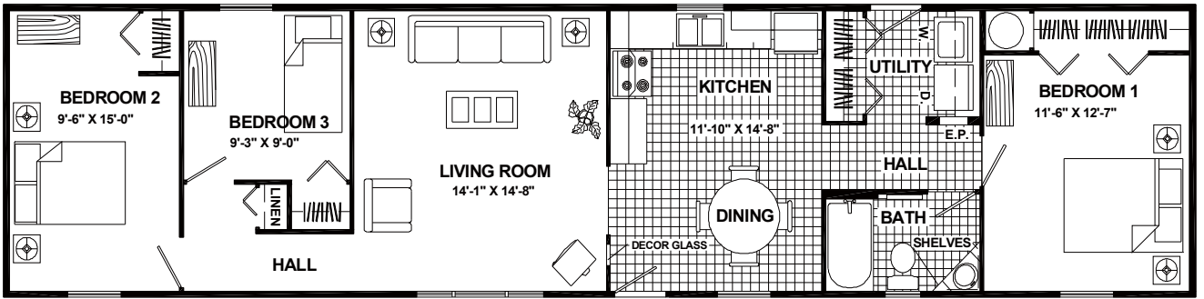
16 X 67 - 3141 (NOT AVAILABLE IN 14' WIDE) 1072 SQ. FT.
